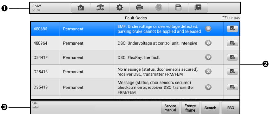
Figure 4-12 Read Codes Screen
