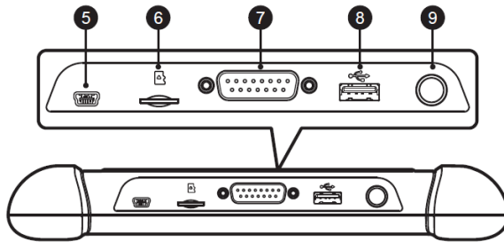
Figure 2-2 Tablet Top View
